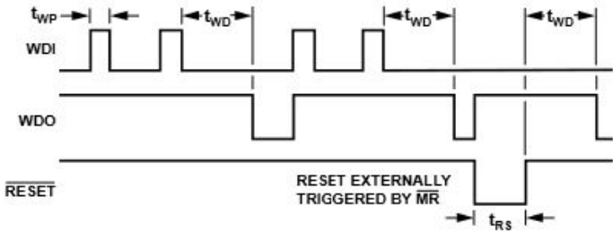
Figure 16. Watchdog Timing
